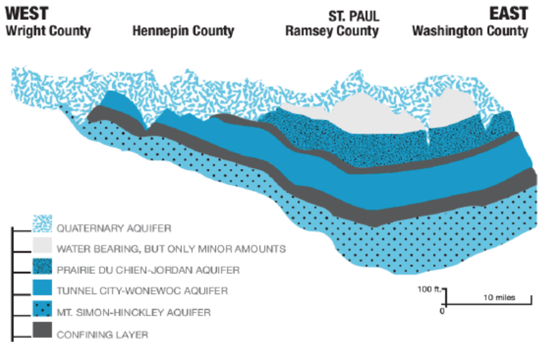
Figure 1.2: Regionally significant aquifers Graphic source: Met Council
