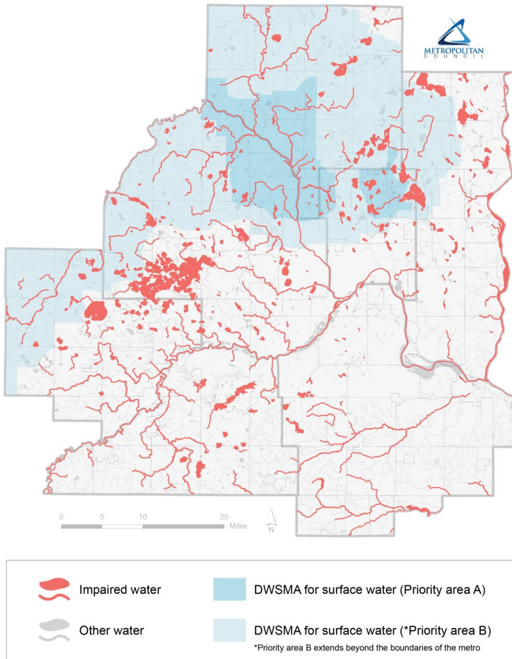
Figure 1.3: Surface Water Drinking Water Supply Management Areas and Impaired Waters
