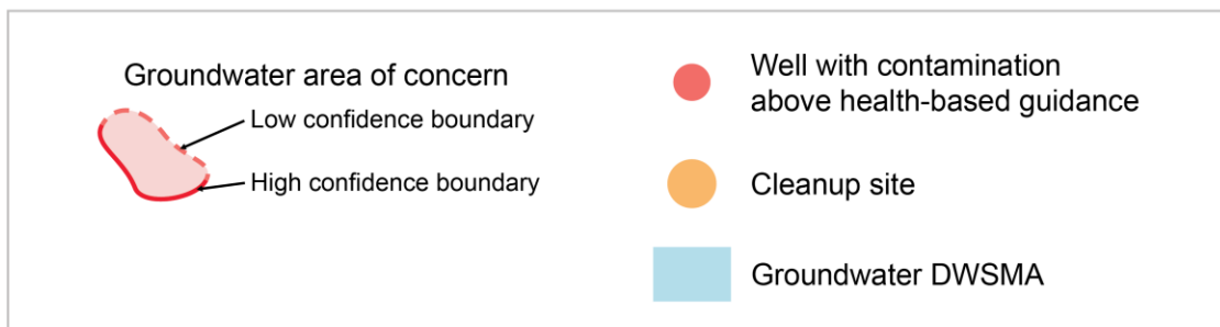
Figure 1.4: Contamination areas and groundwater Drinking Water Supply Management Areas
