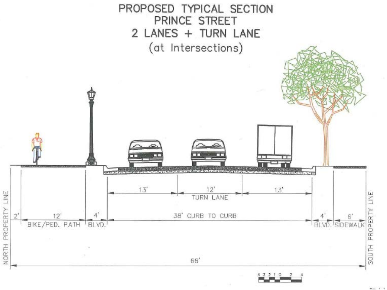
Figure 3: Bruce Vento Regional Trail Realignment Typical Cross-Section
