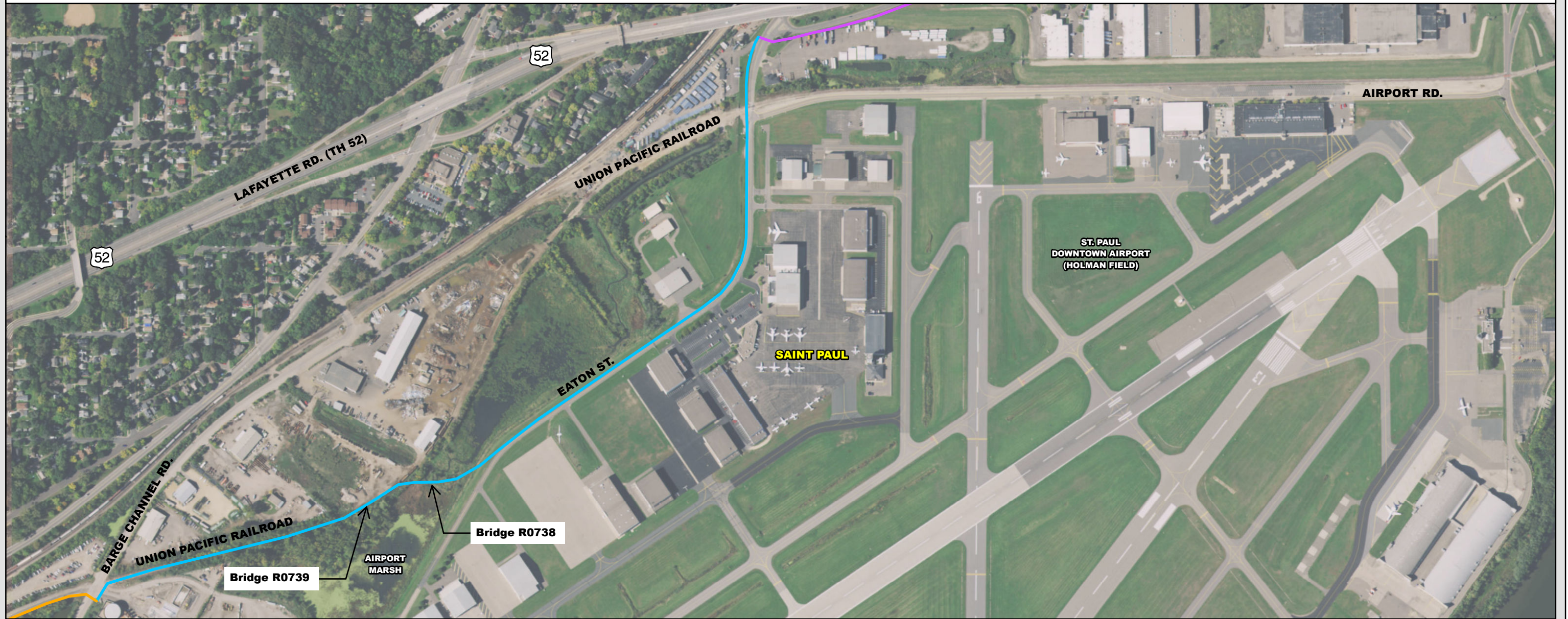
EXHIBIT 1C PROJECT LAYOUT
