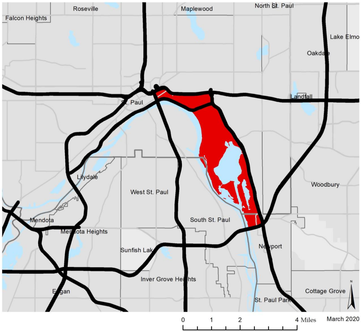
Figure E-1: PM 10 Carbon Monoxide Maintenance Area
