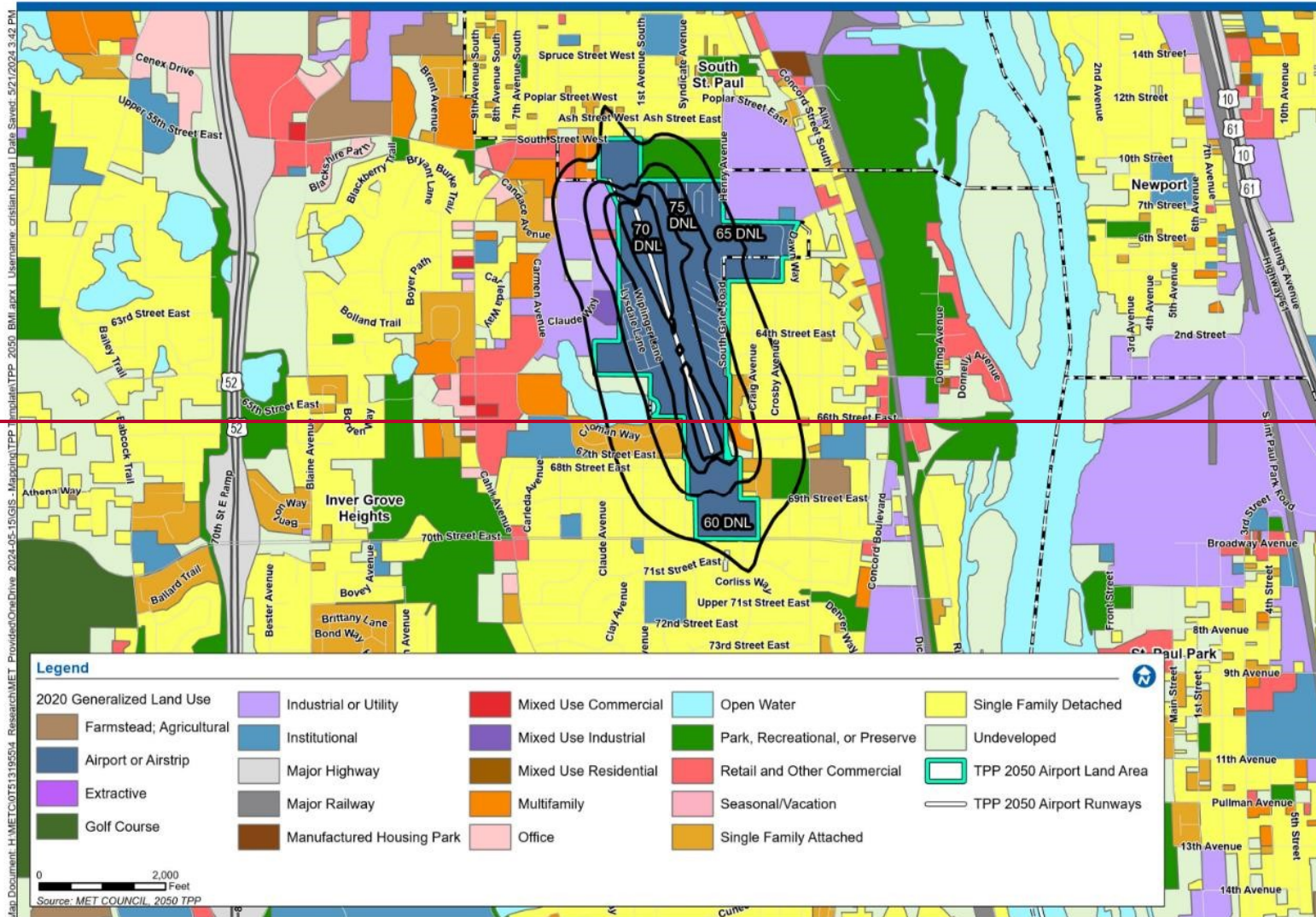
Figure 12 - 2032 Noise Contours
