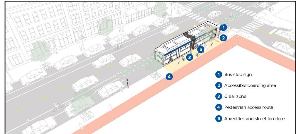
Figure 12 The bus stop clear zone, behind the curb
