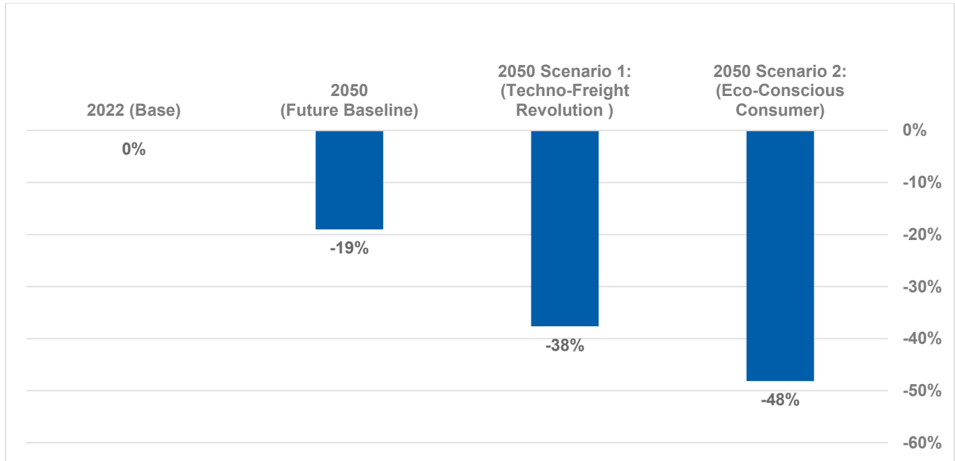
Figure 3. E-Commerce future scenarios: relative change in projected regional greenhouse gas emissions compared to base year 2022 and 2050 baseline conditions 2
