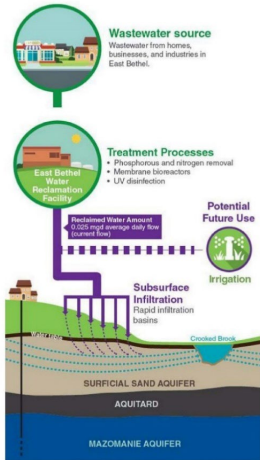
Figure 4: East Bethel water reclamation system
