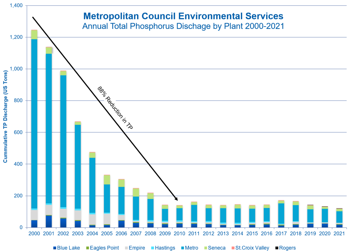
Figure 13: Environmental Services system-wide total phosphorus discharge, 2000-2021
