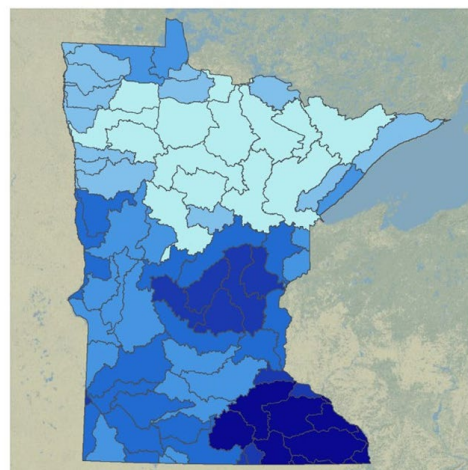
Figure 9: Annual precipitation change, 2000-2019 (Our Minnesota Climate, 2022)
