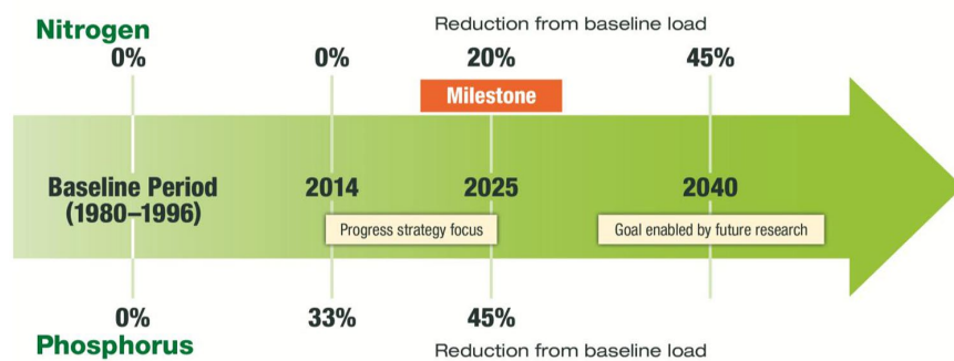
Figure 14: Nutrient reduction timeline for Mississippi River (MPCA, 2014)
