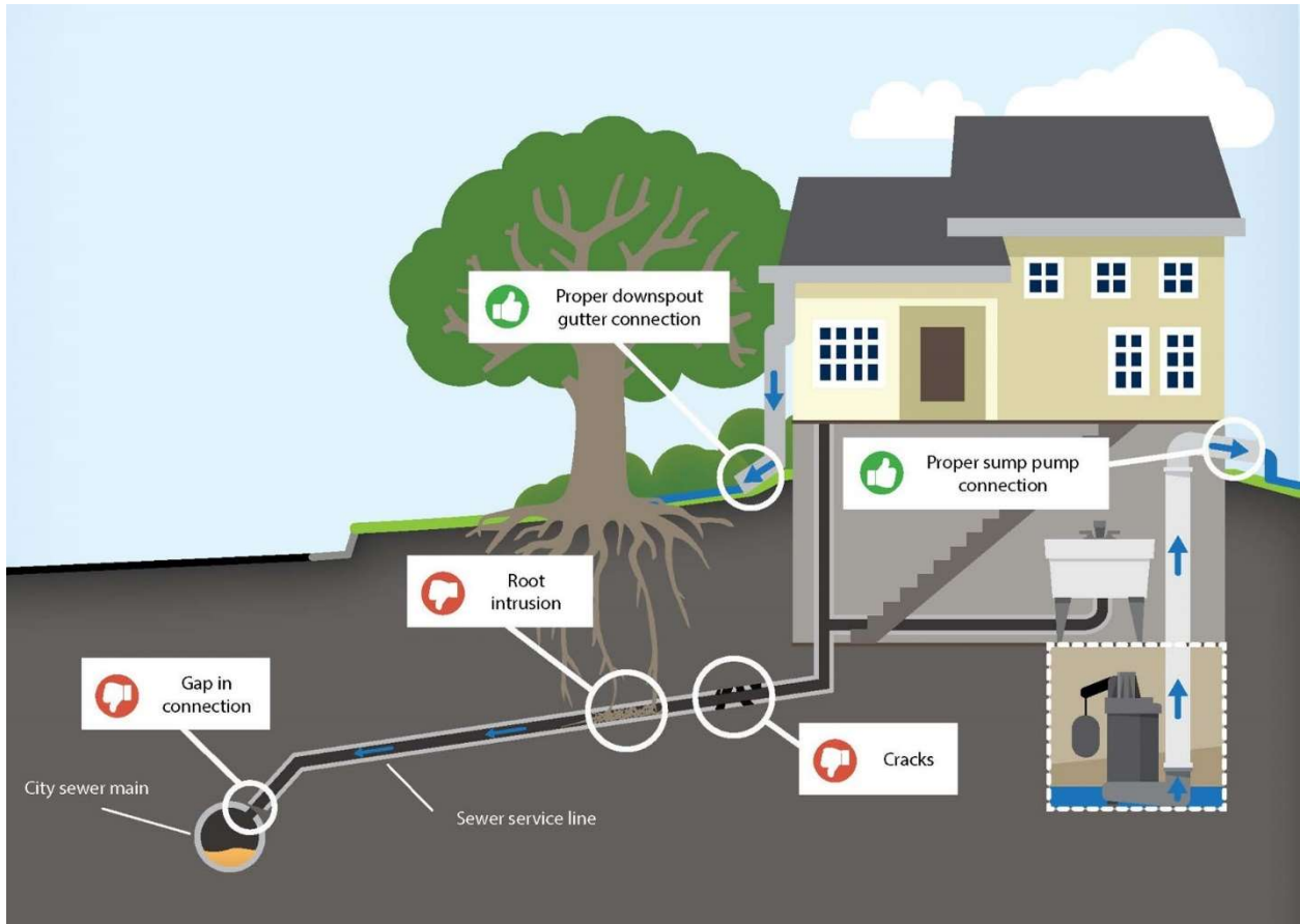
Figure 4: Sources of I/I from private property
