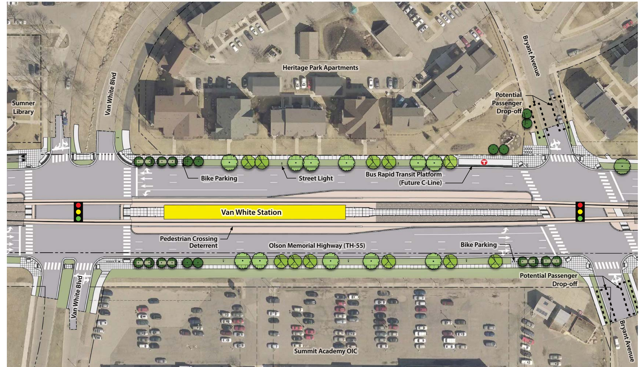
Site Plan
