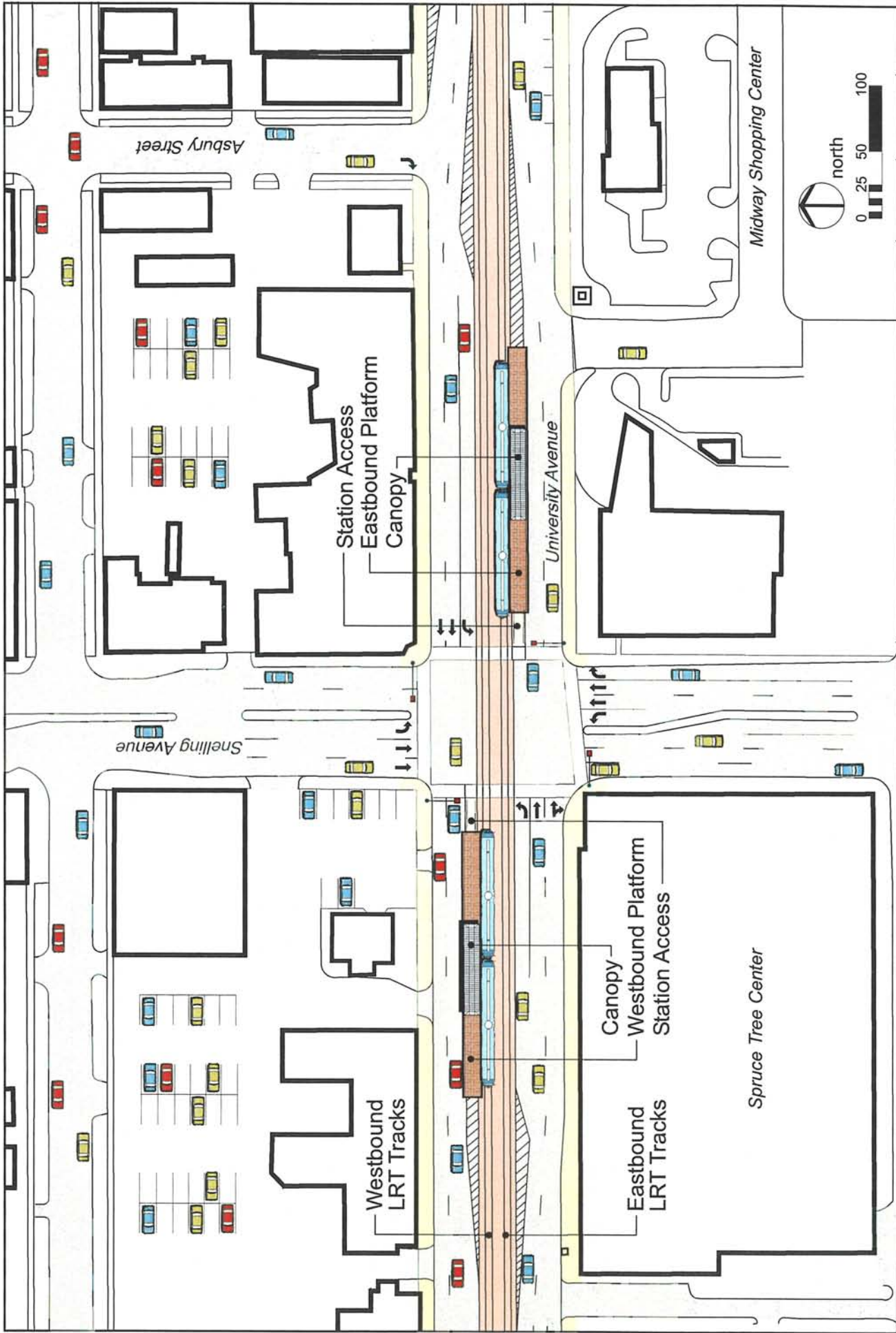
THE CENTRAL CORRIDOR Prototypical LRT Station: Split, Far-Side Platform Snelling Avenue Station Site
