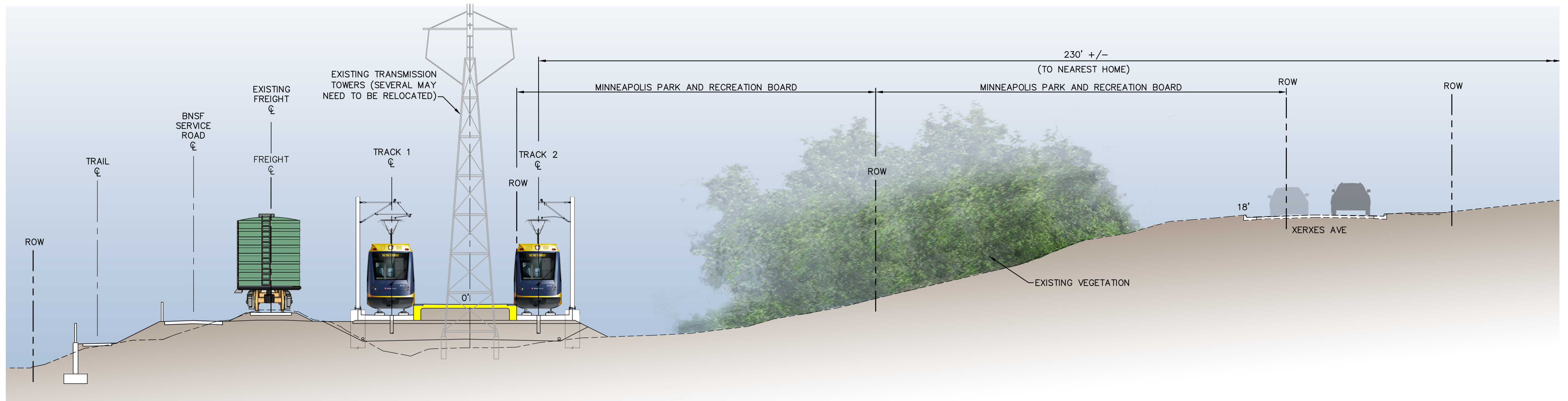
NORTH PLATFORM OPTION
