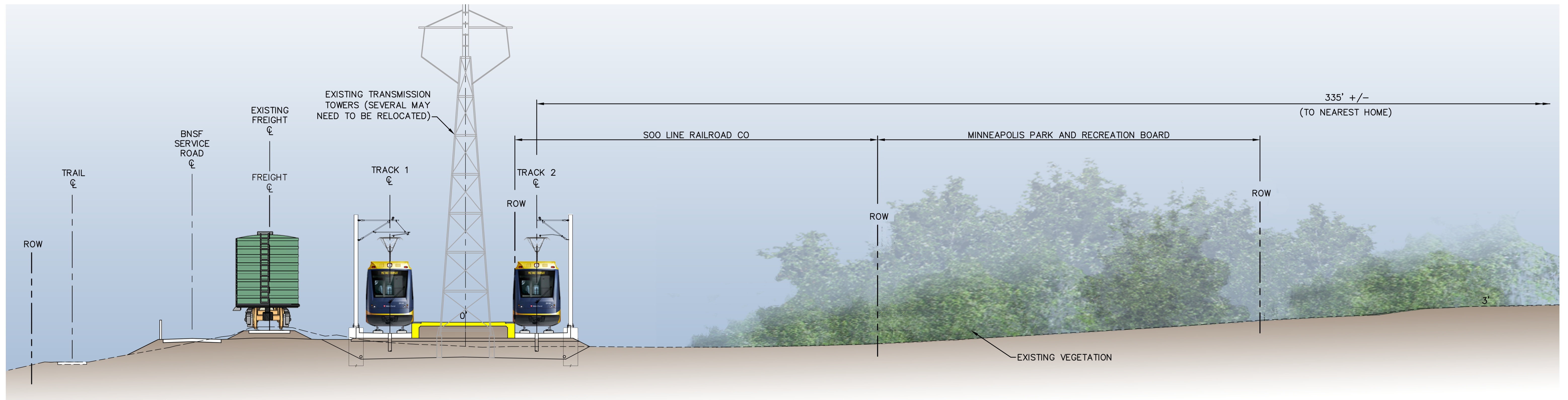
SOUTH PLATFORM OPTION
