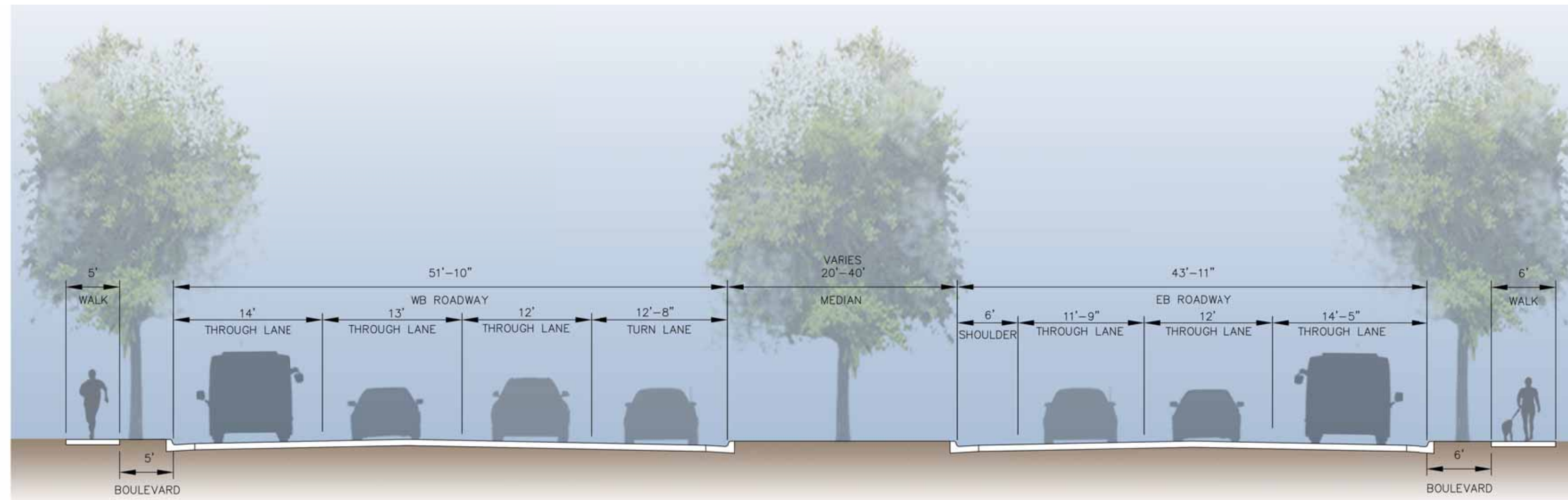
Existing Conditions - Typical Section
