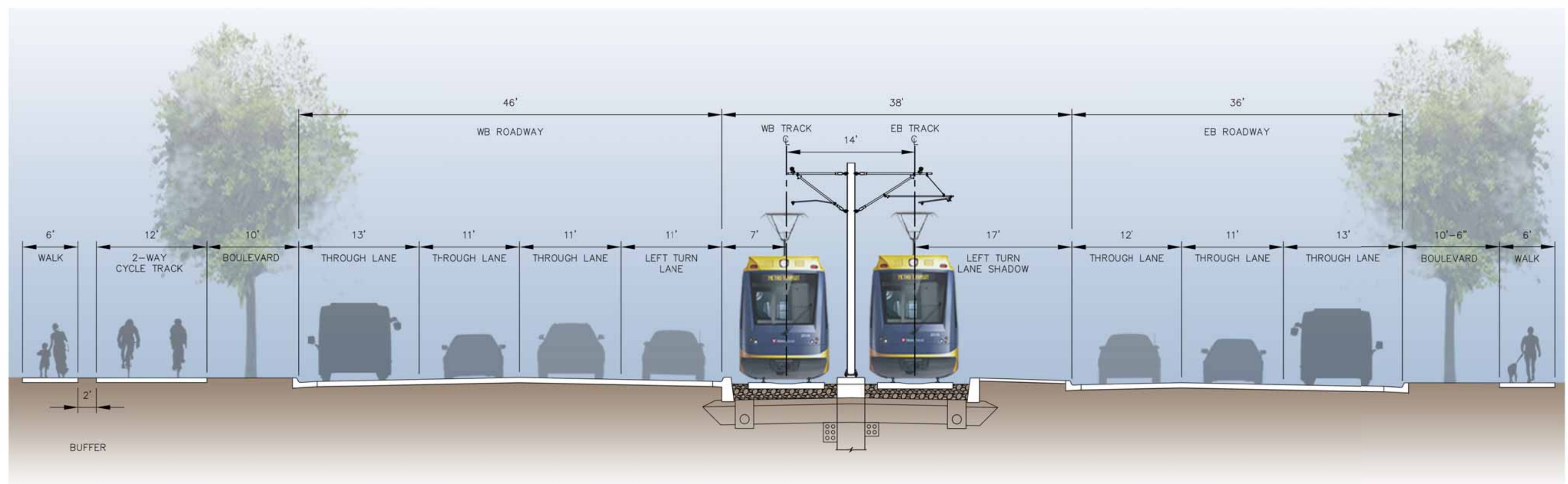
Proposed Conditions - Typical Section
