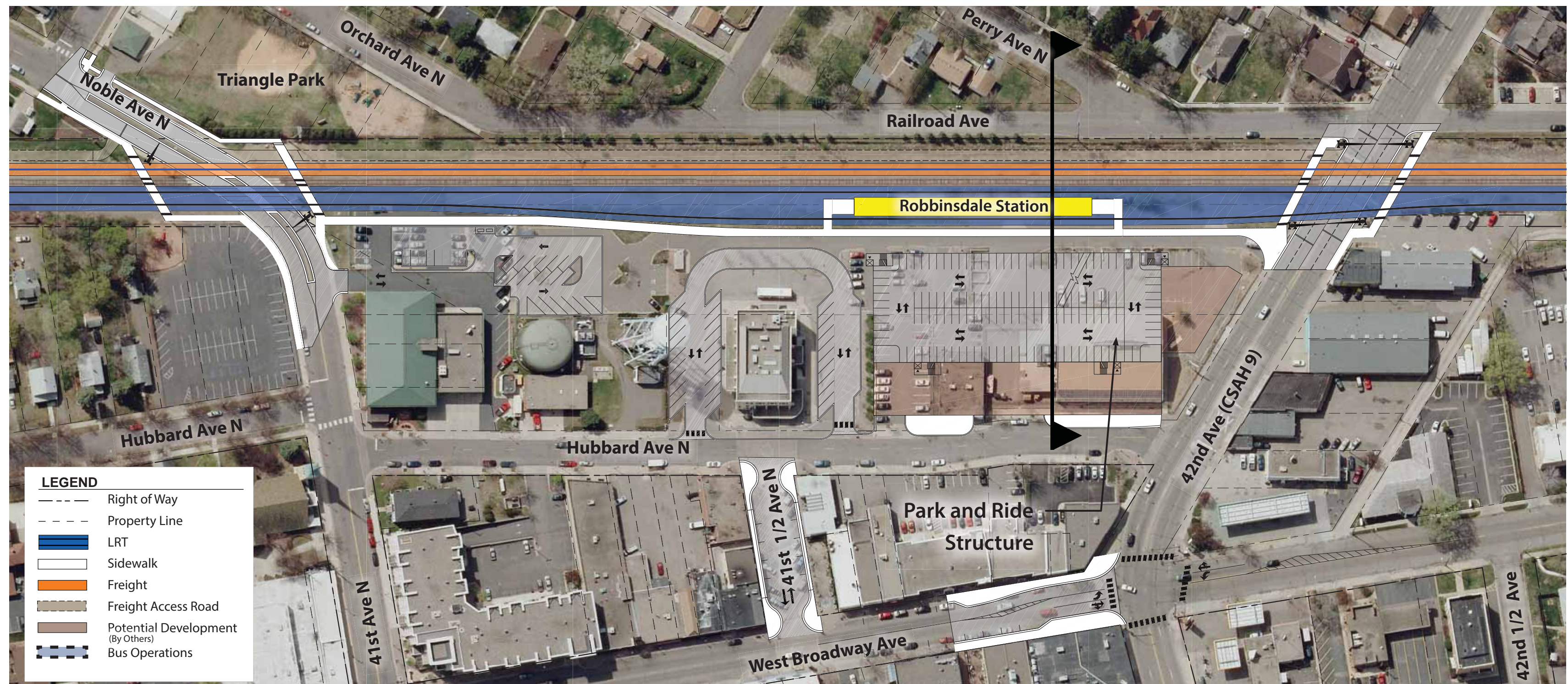
At-Grade Station - Site Plan (Roof Level)
