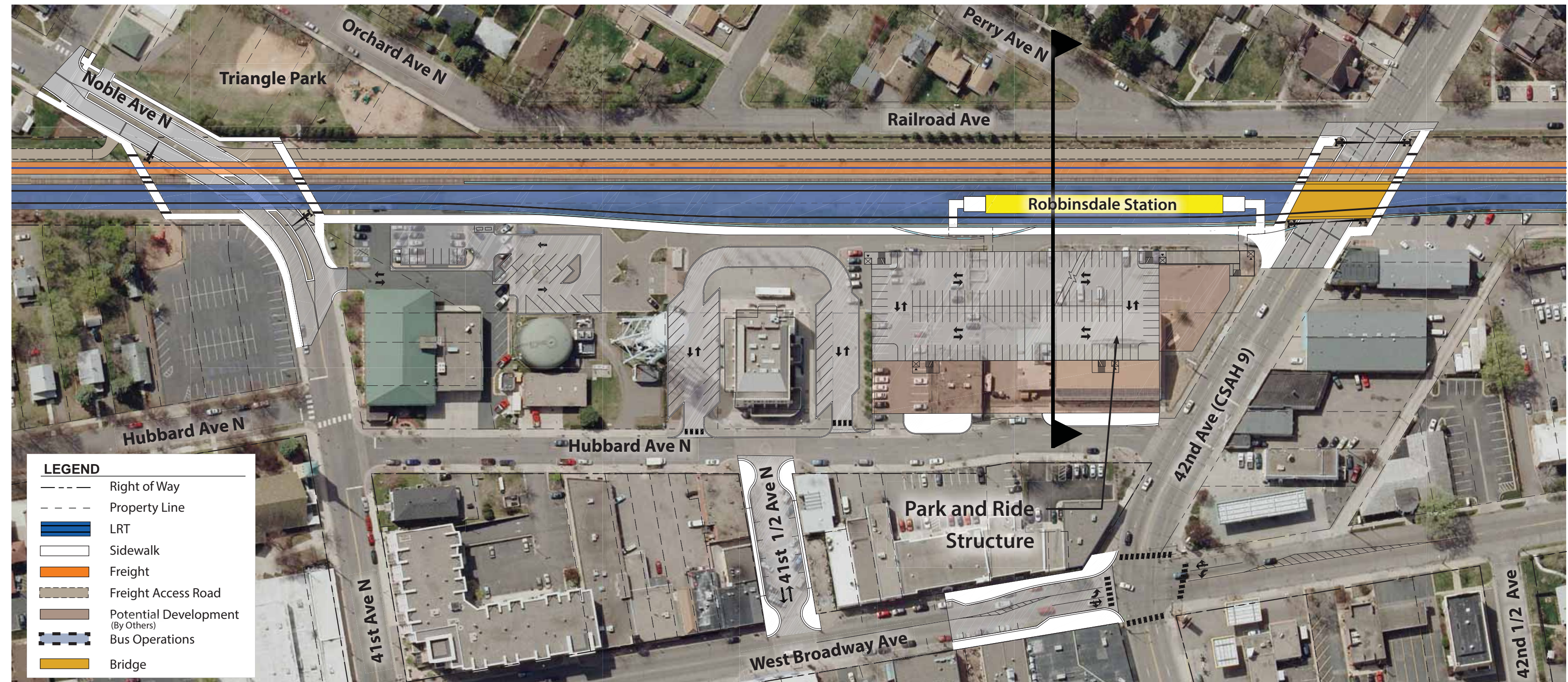
Grade Separated Station - Site Plan (Roof Level)
