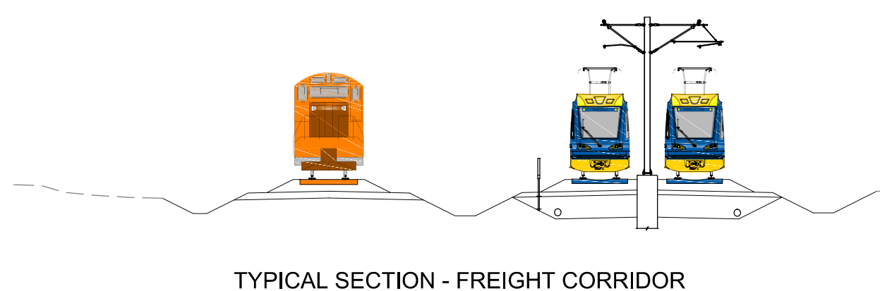
TYPICAL SECTION - FREIGHT CORRIDOR
