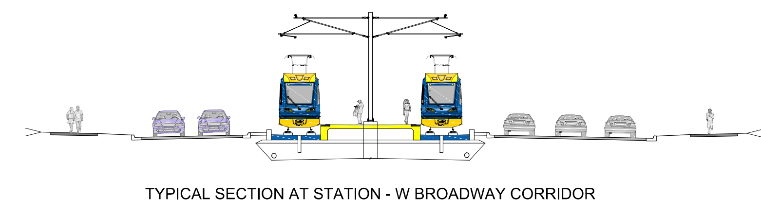
TYPICAL SECTION AT STATION - W BROADWAY CORRIDOR
