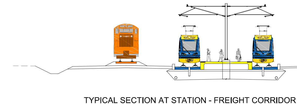
TYPICAL SECTION AT STATION - FREIGHT CORRIDOR
