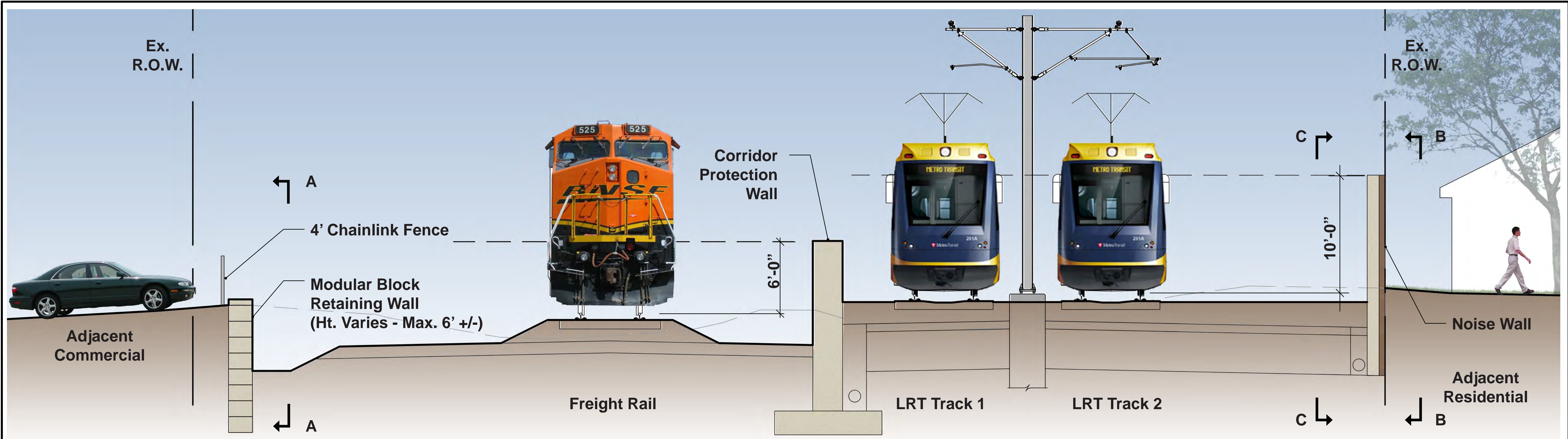
Section View (Looking North)
