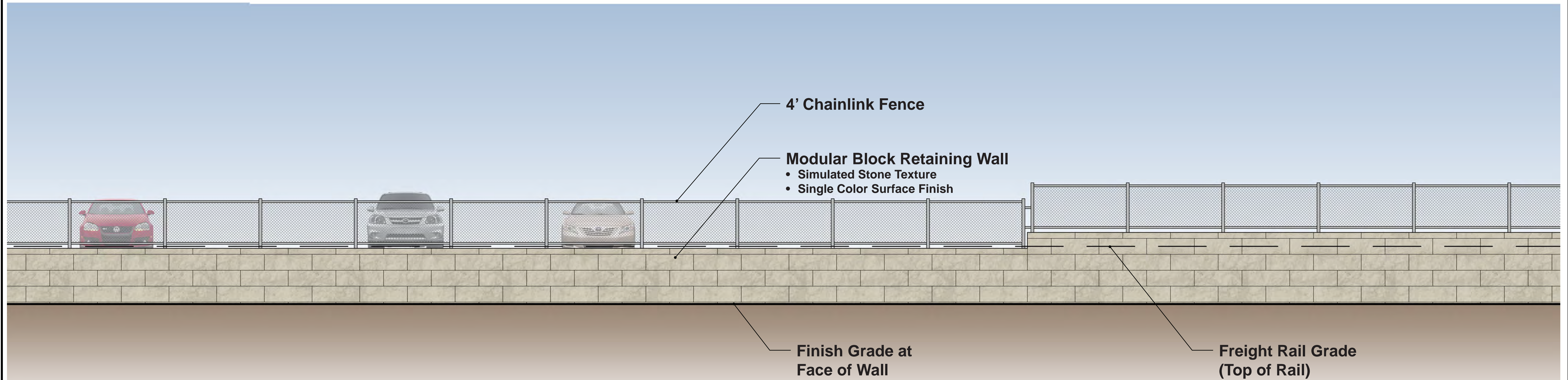
Elevation View A-A (Looking West)
