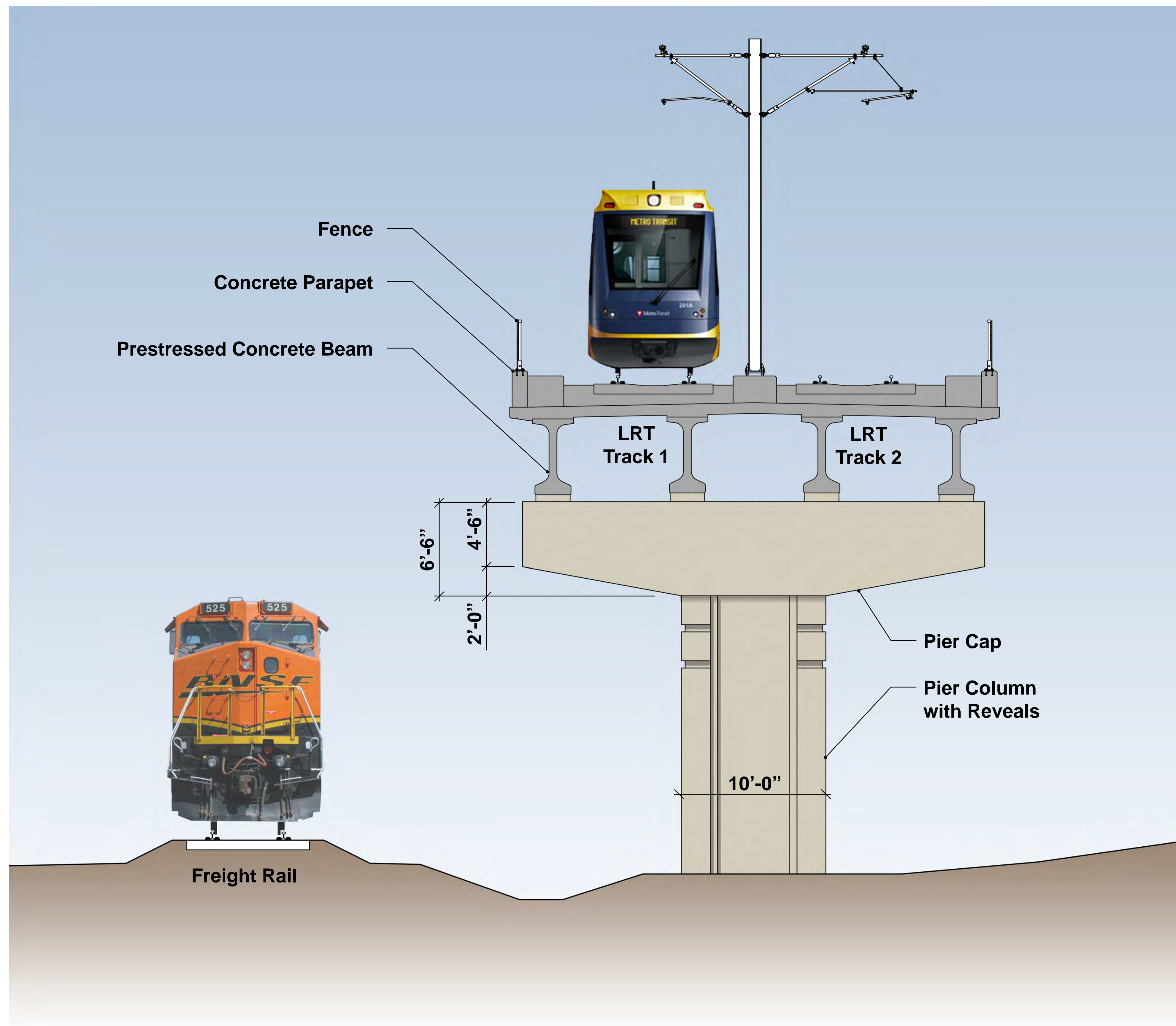
Pier Elevation Detail H-H Pier Form
