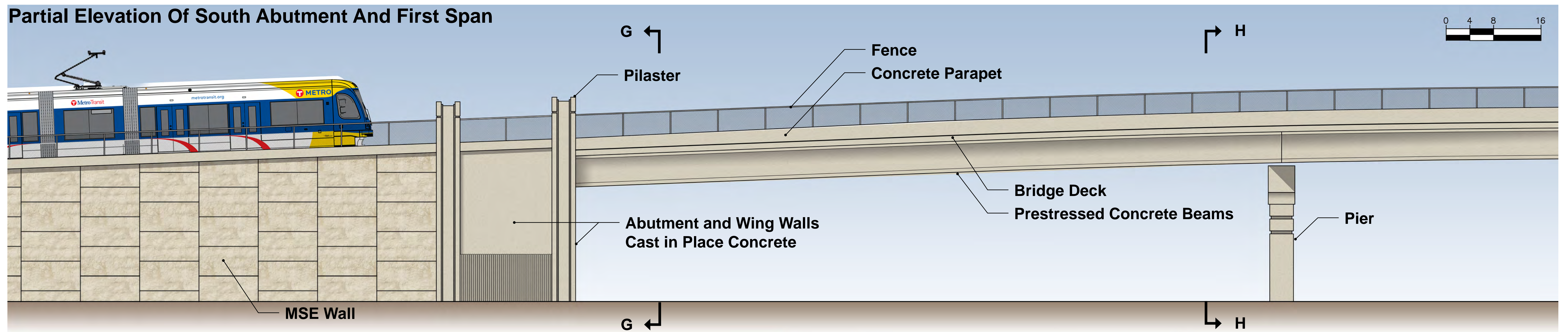
Wing Wall Elevation Detail
