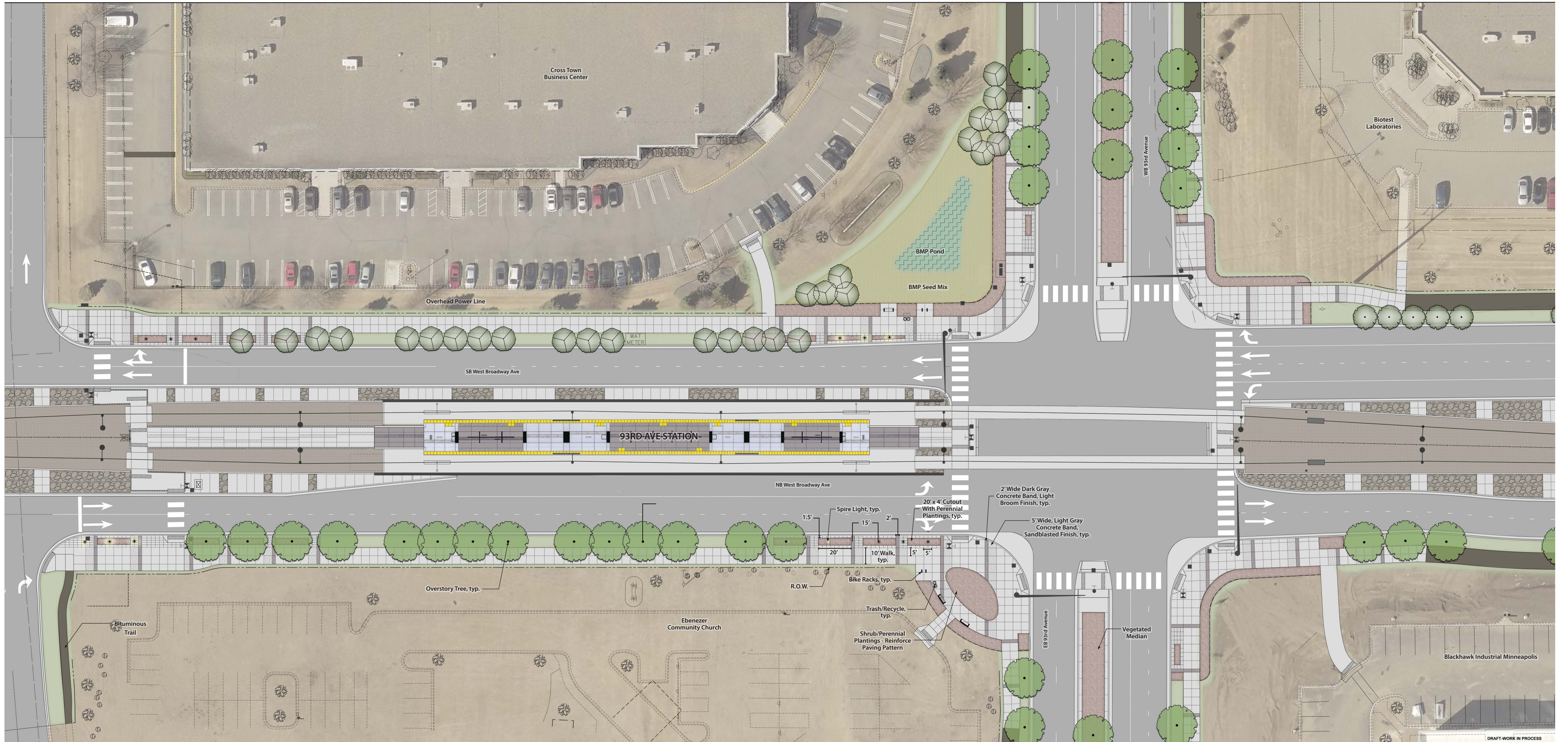
Site Plan
