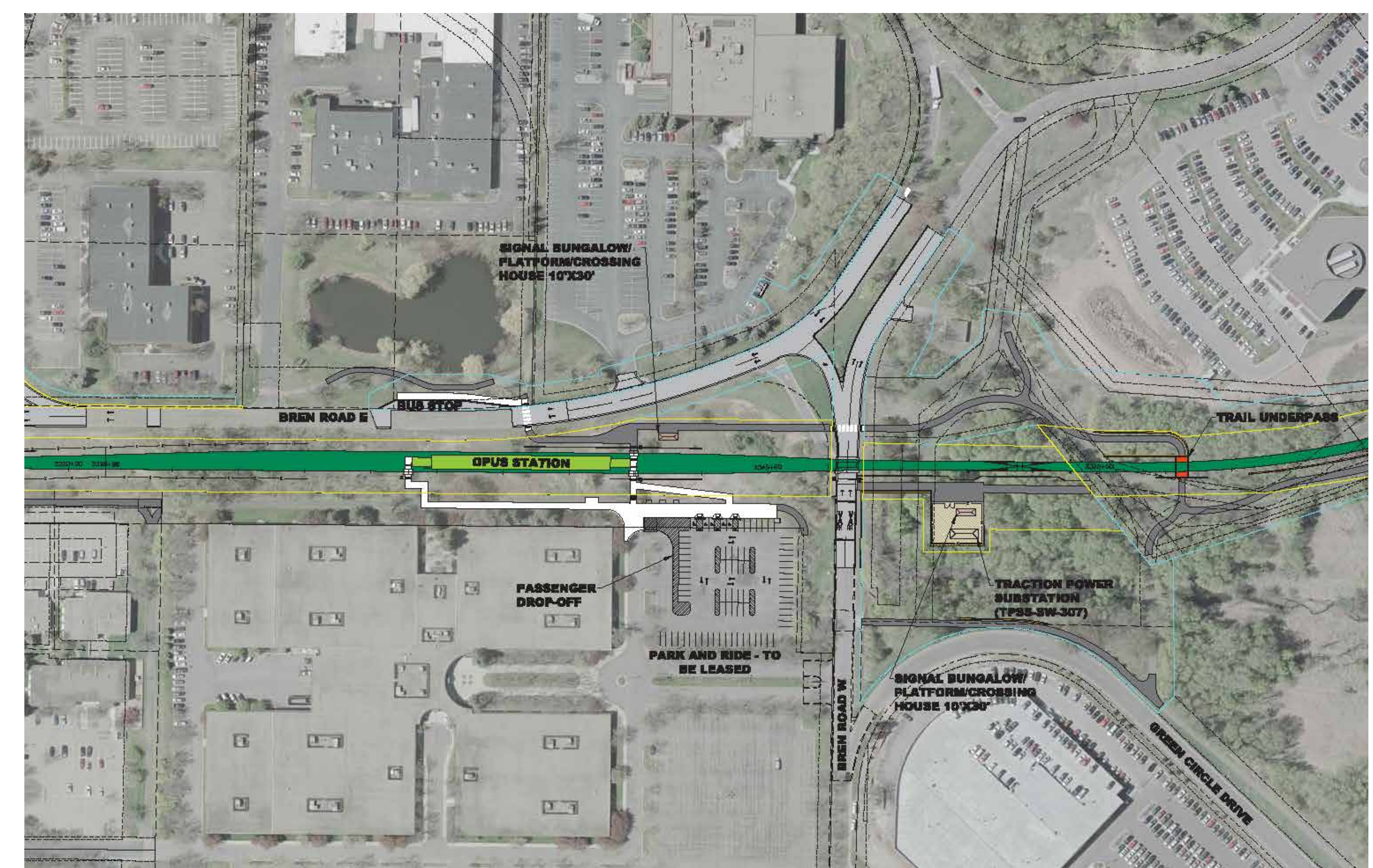
Site plan
