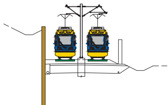
TYPICAL SECTION AT RETAINING WALL
