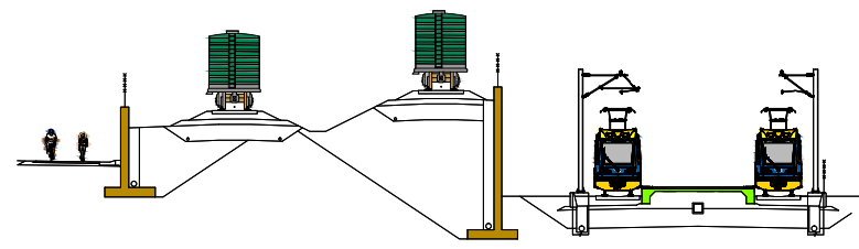
TYPICAL SECTION AT PLATFORM
