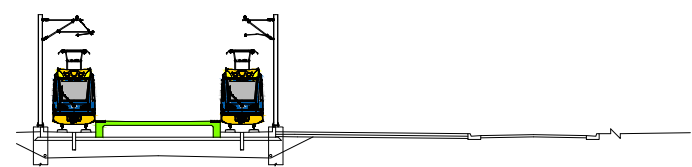
TYPICAL SECTION AT STATION
