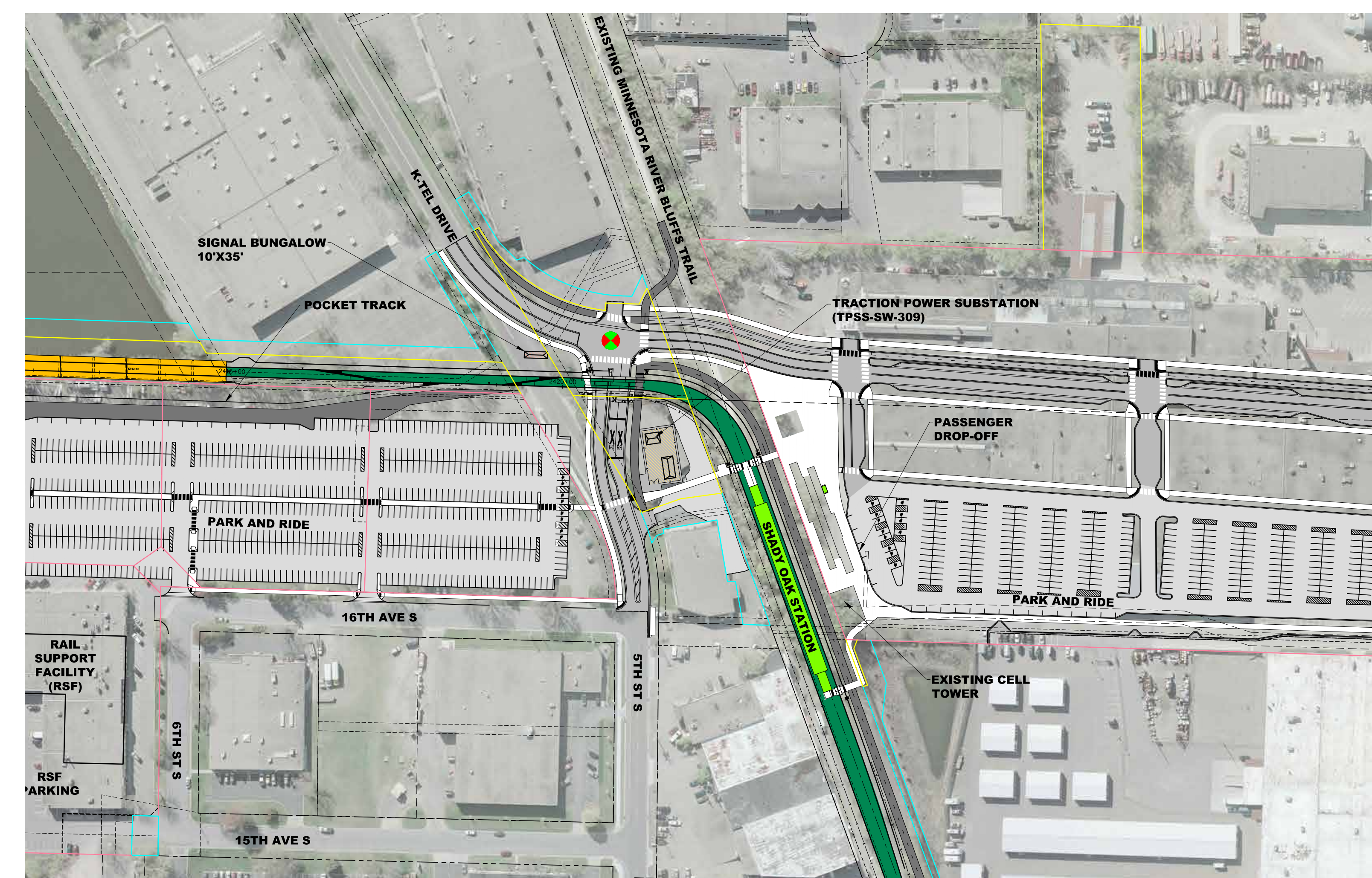
Site plan
