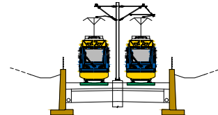
TYPICAL SECTION AT TUNNEL TYPICAL SECTION AT RETAINING WALL
