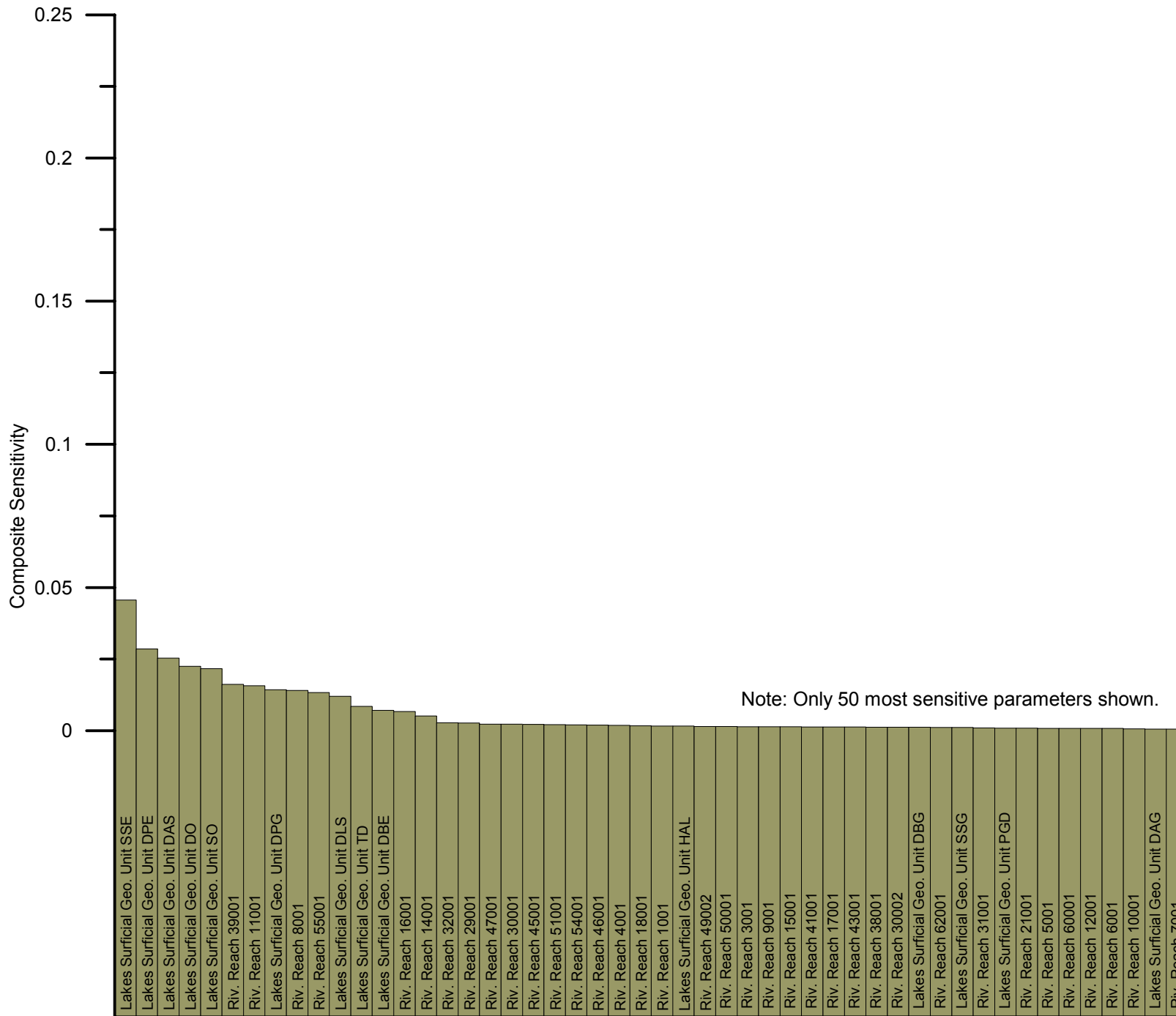
Figure B10 Parameter Sensitivities River and Lake Vertical Hydraulic Conductivity Entire Model Domain
