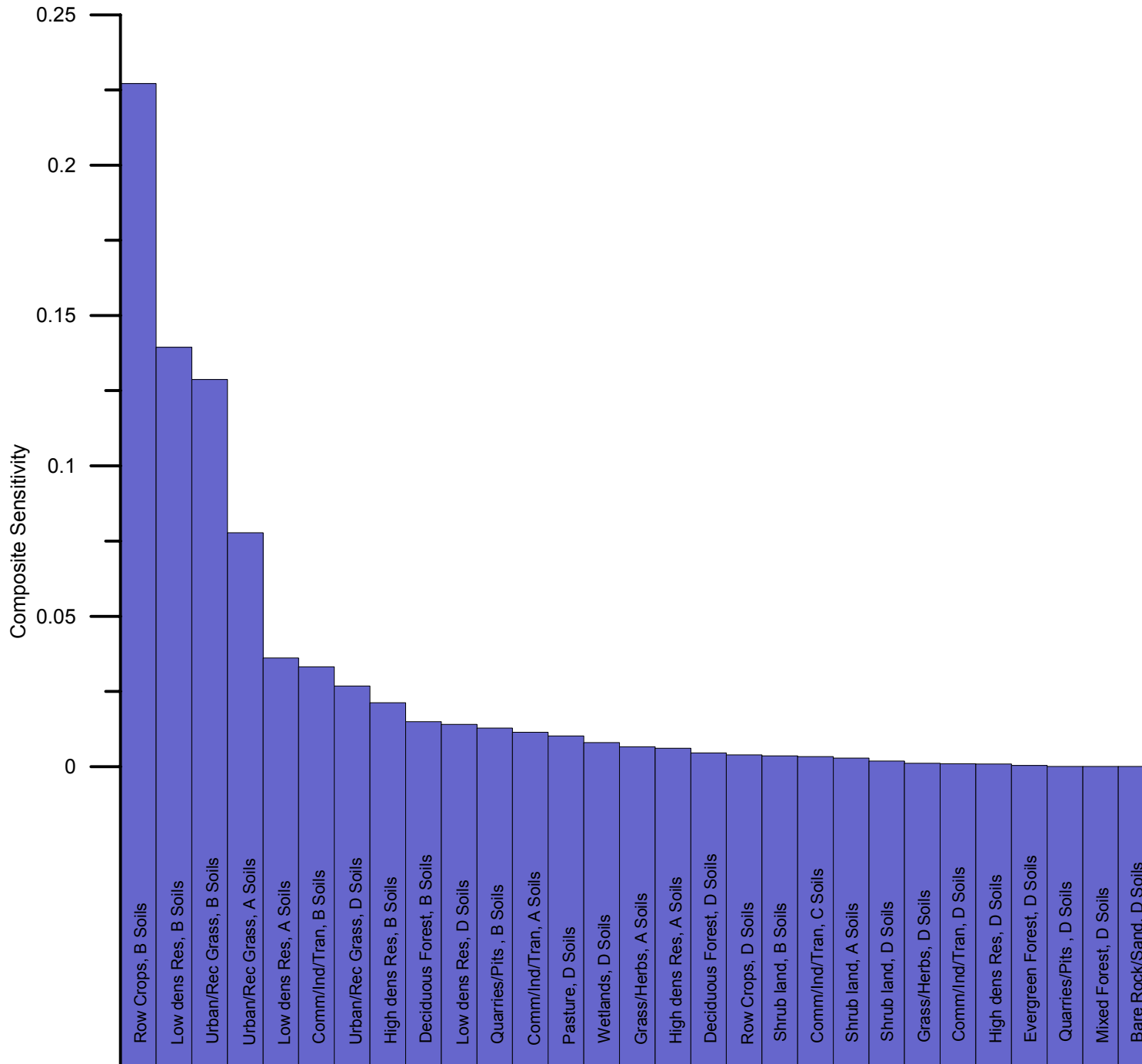
Figure B9 Parameter Sensivities Recharge Multiplier Entire Model Domain
