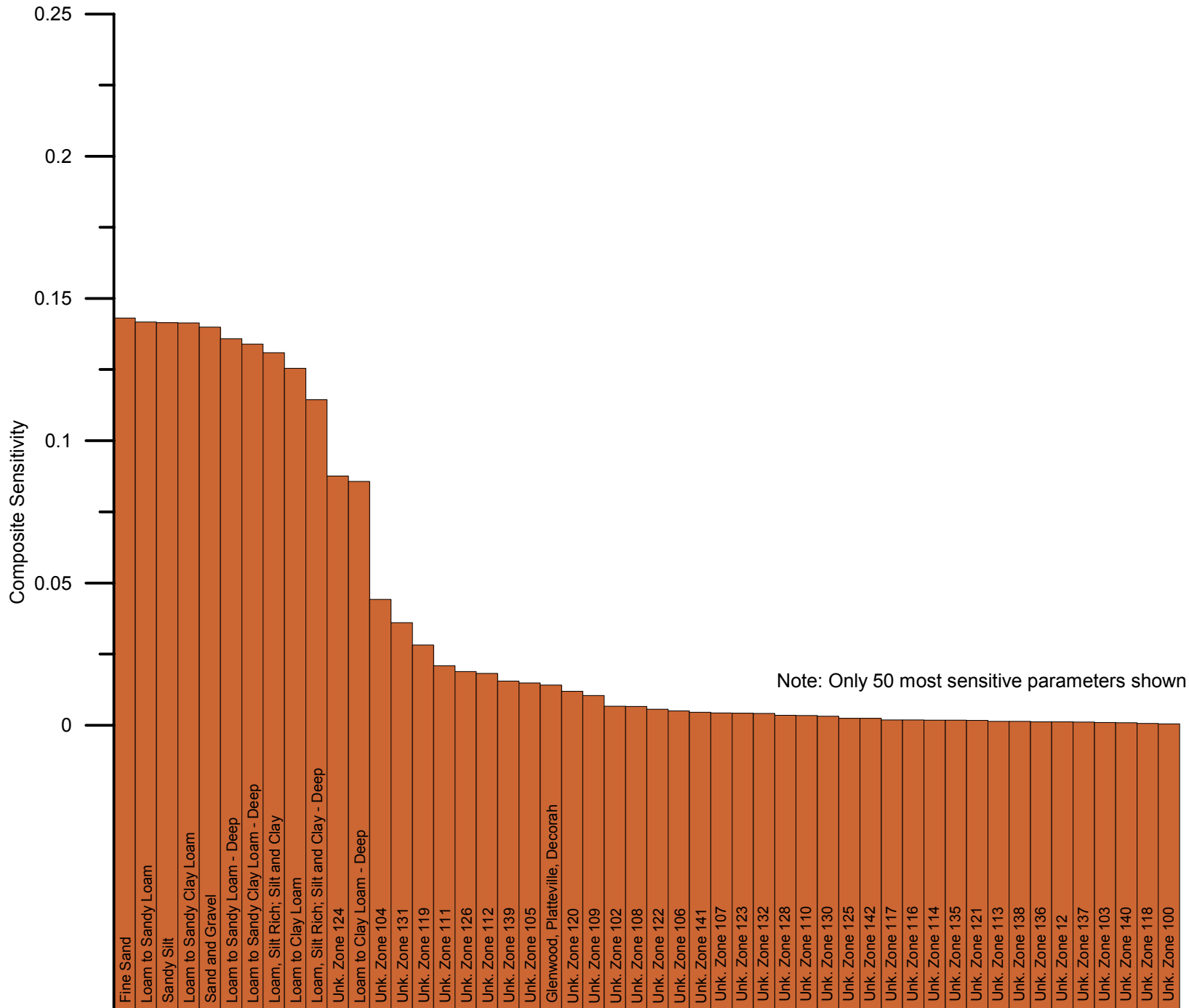
Figure B8 Parameter Sensitivities Quaternary Vertical Hydraulic Conductivity Entire Model Domain
