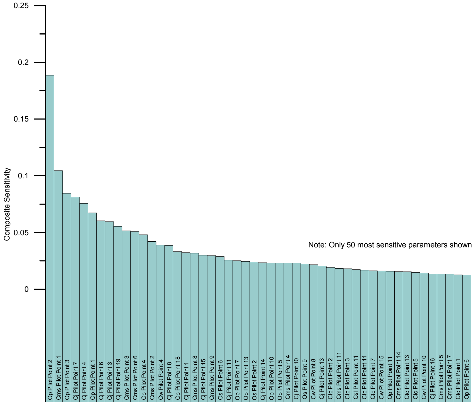
Figure B2 Parameter Sensitivities Bedrock Horizontal Hydraulic Conductivity Entire Model Domain
