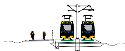
TYPICAL SECTION AT GRADE
