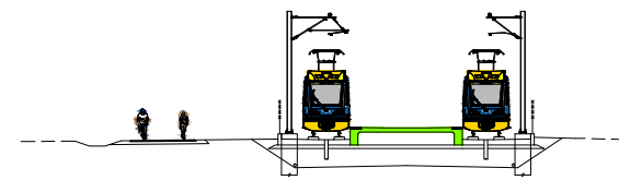
TYPICAL SECTION AT STATION
