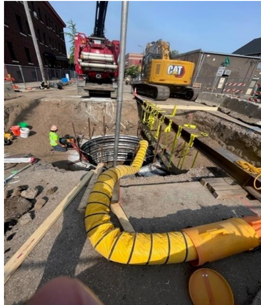
Excavation opened Gas main supported
