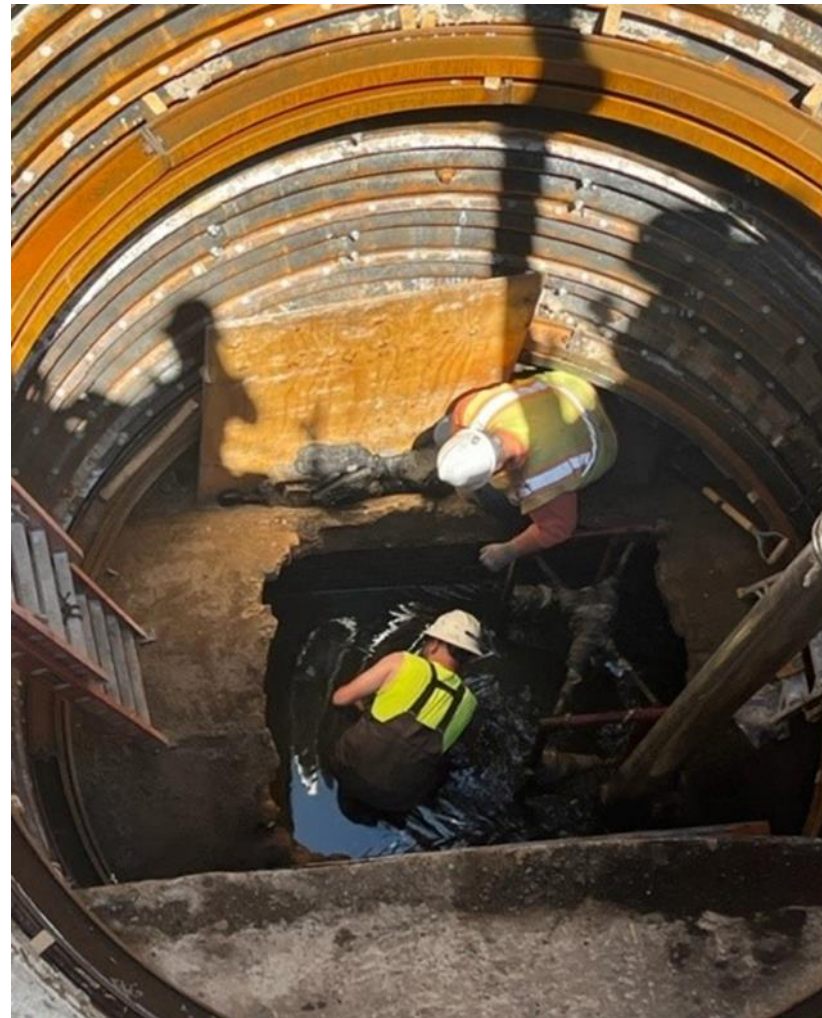
MH/Pipe connection cleaned
