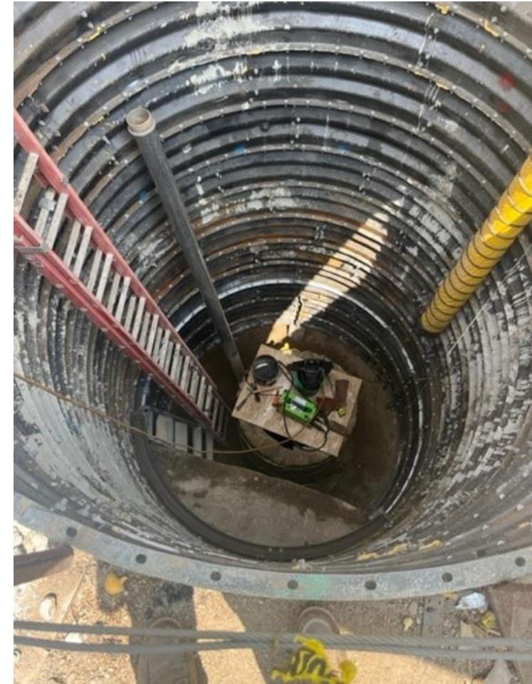
Retention system installed Storm sewer exposed
