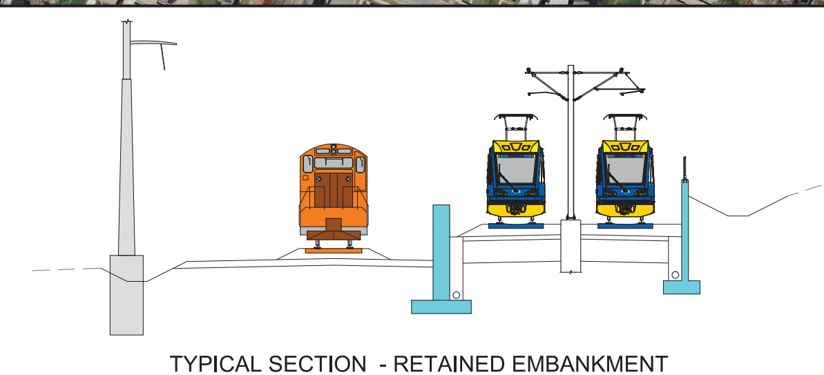
TYPICAL SECTION - RETAINED EMBANKMENT
