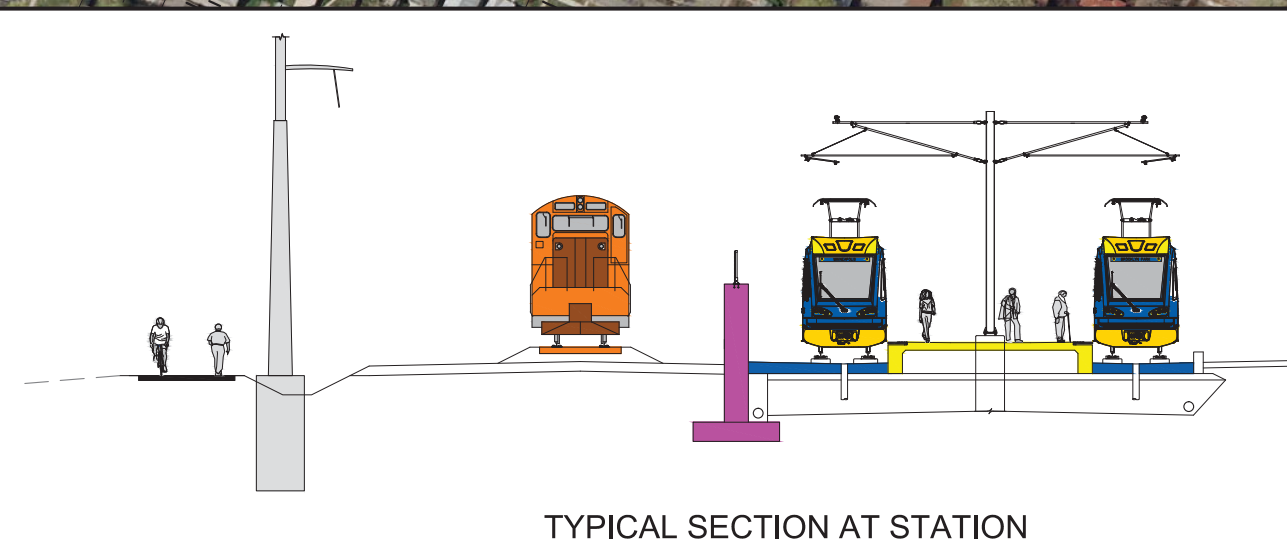
TYPICAL SECTION AT STATION
