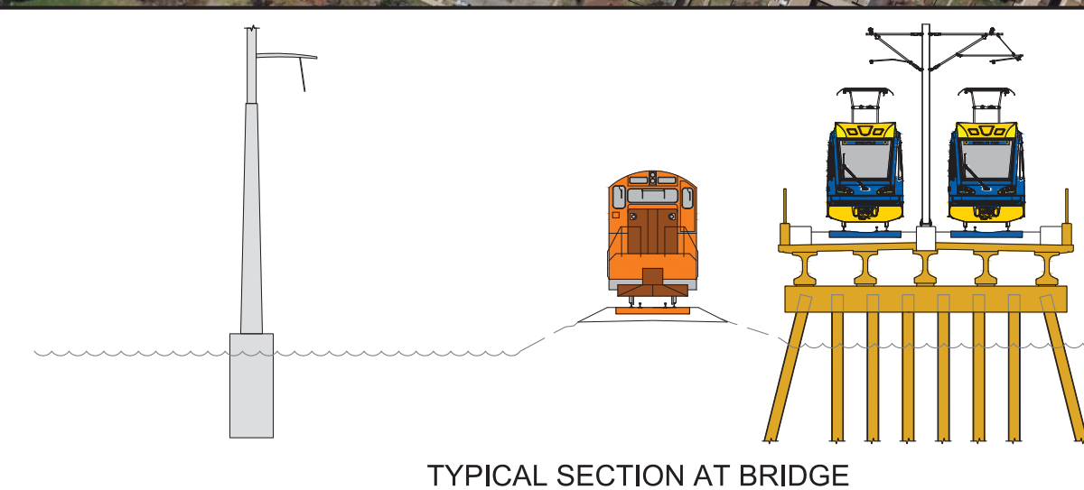
TYPICAL SECTION AT BRIDGE
